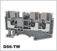
DS6-TW 1000V/41A 0.5-6mm 2 UL 600V/40A 20-8AWG T/W/End plate 8.2/57.7/1.5mm
