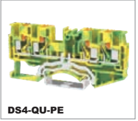
DS4-QU-PE — 0.2-6mm 2 — 24-10AWG T/W/End plate 6.2/77/2.2mm
