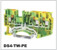
DS4-TW-PE — 0.2-6mm 2 — 24-10AWG T/W/End plate 6.2/66.5/2.2mm
