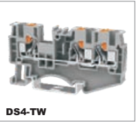
DS4-TW 800V/32A 0.2-6mm 2 600V/30A 24-10AWG T/W/End plate 6.2/66.5/2.2mm
