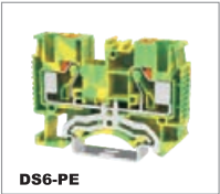
DS6-PE — 0.5-10mm 2 — 20-8AWG T/W/End plate 8.2/57.7/1.5mm
