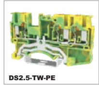
DS2.5-TW-PE — 0.2-4mm 2 — 26-12AWG T/W/End plate 5.2/60.5/2.2mm
