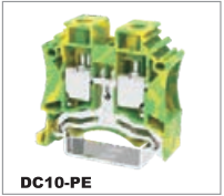
DC10-PE — 0.5-16mm 2 — 20-6AWG T/W/End plate 10/43.9/1.5mm
