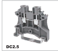
DC2.5 800V/24A 0.2-4mm 2 600V/25A 26-12AWG T/W/End plate 5.1/44.5/1.5mm
