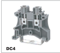
DC4 1000V/32A 0.2-6mm 2 600V/30A 22-10AWG T/W/End plate 6.1/44.5/1.5mm
