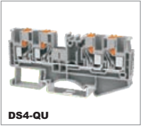
DS4-QU 800V/32A 0.2-6mm 2 600V/30A 24-10AWG T/W/End plate 6.2/77/2.2mm
