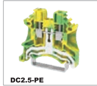
DC2.5-PE — 0.2-4mm 2 — 26-12AWG T/W/End plate 5.1/44.5/1.5mm
