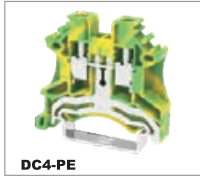
DC4-PE — 0.2-6mm 2 — 22-10AWG T/W/End plate 6.1/44.5/1.5mm
