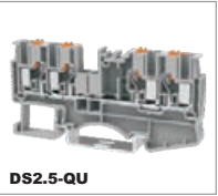
DS2.5-QU 800V/24A 0.2-4mm 2 600V/20A 26-12AWG T/W/End plate 5.2/72.20/2.2mm
